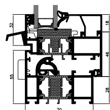
cross-section of MB-70HI window
