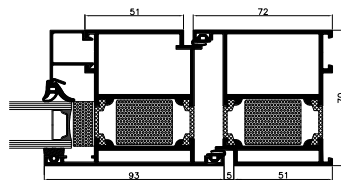
cross-section of MB-70HI door
